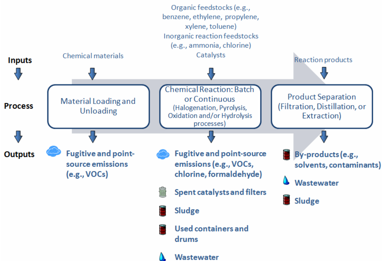
Figure 1: Basic Organic Chemical Manufacturing Processes
