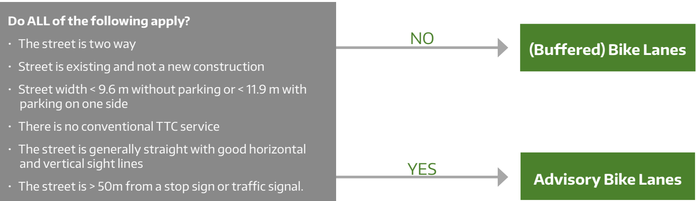
Figure 3.29 Conventional or buffered bike lanes and advisory lane facility decision matrix
